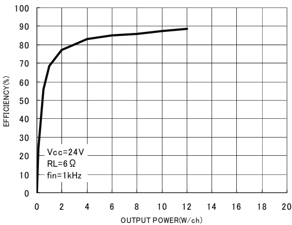
Fig. 17 Output power—Efficiency ( R_L=6\Omega )
