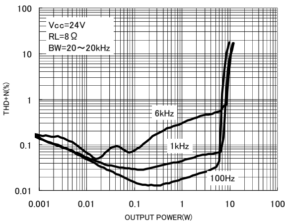
Fig.3 Output power—THD+N
