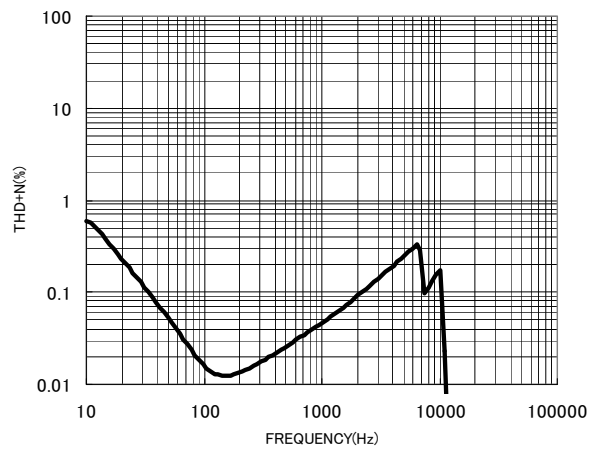
Fig.4 Frequency—THD+N
