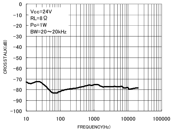
Fig.6 Frequency—Crosstalk
